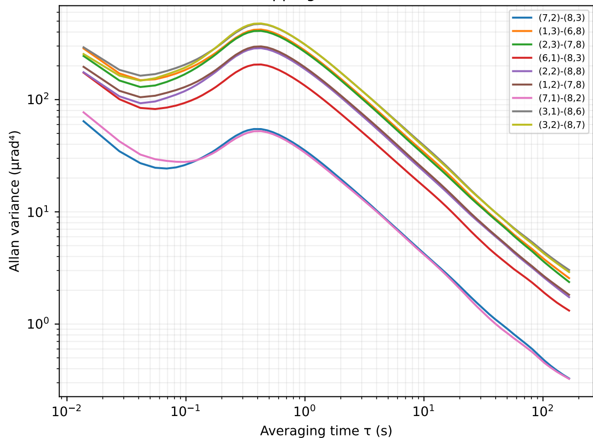
Overlapping Allan variance
